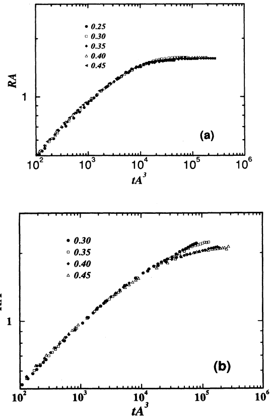
FIG. 5. (a) Scaled domain size RA vs scaled time tA^3 for T = 0 , using \beta = 1 and \gamma = 3 in the scaling relation Eq. (2.13). The collapse onto a single curve further confirms our scaling hypothesis. (b) Same plot as (a) using simulations with T > 0 .
